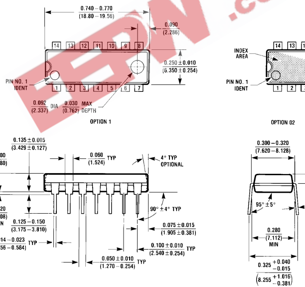
14-Lead Molded Dual-In-Line Package (N) Order Number DM74LS125AN NS Package Number N14A
