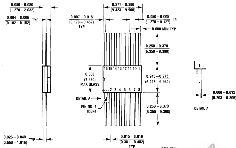
16-Lead Ceramic Flat Package (W) Order Number 54LS138FMB, 54LS139FMB, DM54LS138W or DM54LS139W NS Package Number W16A
