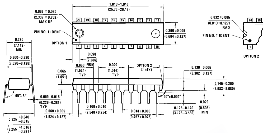
20-Lead Molded Dual-In-Line Package (N) Order Numbers DM74LS465N/DM81LS95AN, DM74LS466N/DM81LS96AN, DM74LS467N/DM81LS97AN or DM74LS468N/DM81LS98AN NS Package Number N20A
