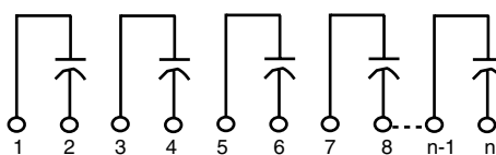
Isolated Capacitor Sections
