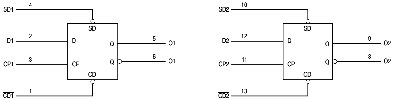
Figure 2. Logic Diagram
