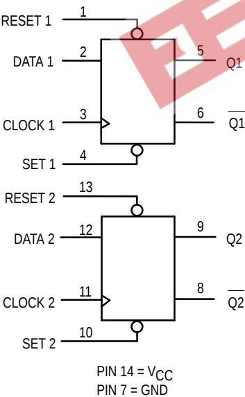
LOGIC DIAGRAM
