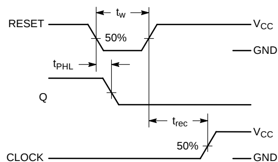
Figure 5. Switching Waveform
