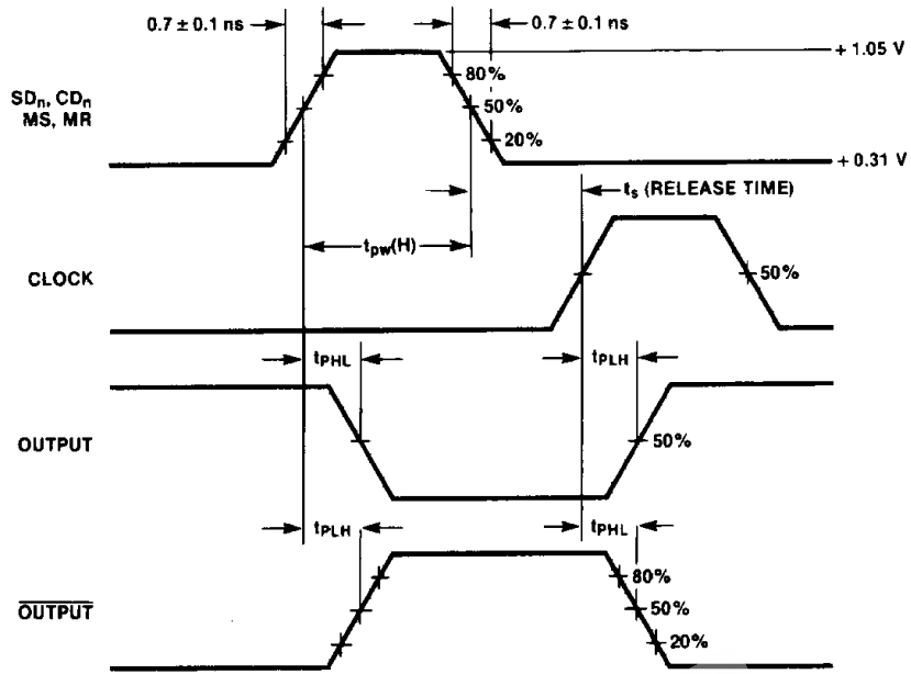
FIGURE 4. Propagation Delay (Reset)
