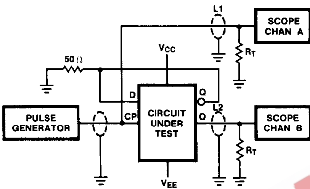
FIGURE 2. Toggle Frequency Test Circuit
