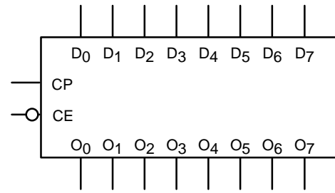
Figure 2. LOGIC SYMBOL
