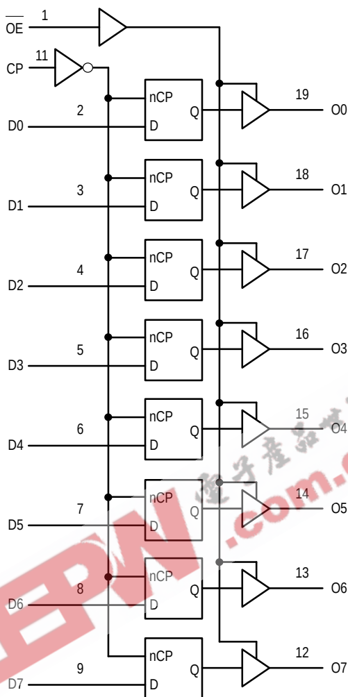
LOGIC DIAGRAM
