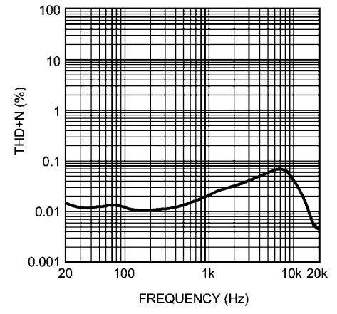
THD+N vs Frequency Single-ended Input, Speaker Mode 2 V_{DD} = 3.6V, P_{OUT} = 450mW/Ch, R_L = 8\Omega
