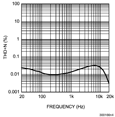
THD+N vs Frequency Single-ended Input, Headphone Mode 2 V_{DD} = 3.6V, P_{OUT} = 30mW, R_L = 16\Omega
