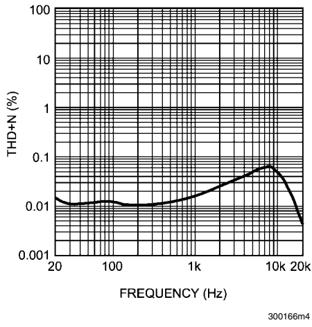
THD+N vs Frequency Differential Input, Headphone Mode 2 V_{DD} = 3.6V, P_{OUT} = 30mW/Ch, R_L = 32\Omega
