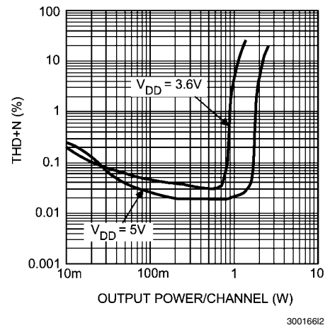
THD+N vs Output Power Differential Input, Speaker Mode 2 A_V = 0dB, R_L = 4\Omega, f = 1kHz
