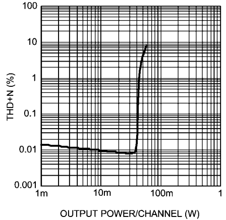
THD+N vs Output Power Differential Input, Headphone Mode 2 V_{DD} = 3.6\text{V} , A_V = 0\text{dB} , R_L = 32\Omega , f = 1\text{kHz}
