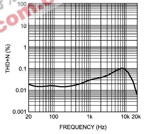
THD+N vs Frequency Single-ended Input, Speaker Mode 2 V_{DD} = 3.6V, P_{OUT} = 650mW/Ch, R_L = 4\Omega
