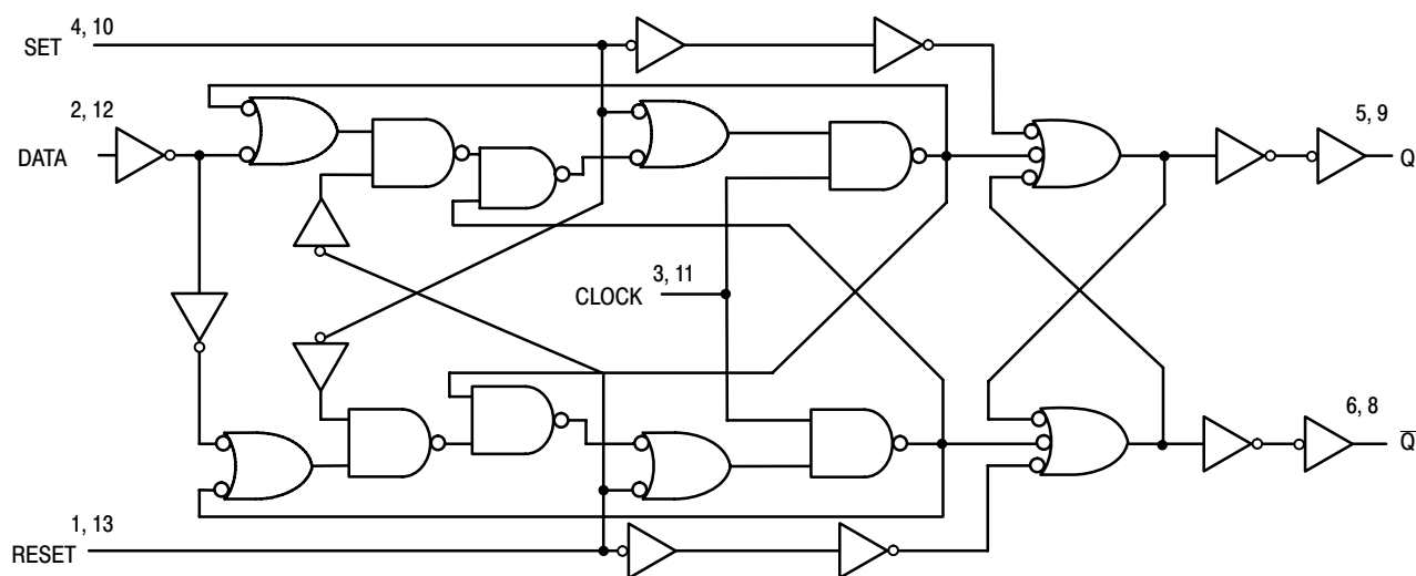
Figure 5. EXPANDED LOGIC DIAGRAM
