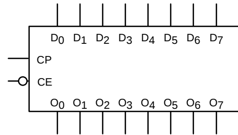
Figure 2. LOGIC SYMBOL
