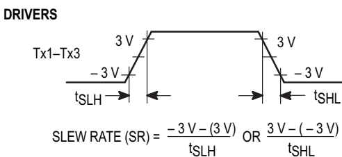
Figure 3. Slew-Rate Characterization
