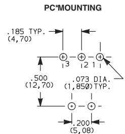
PC MOUNTING
