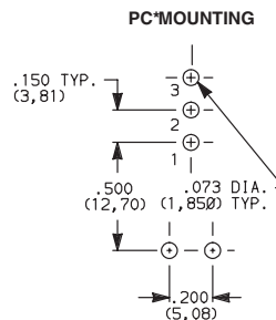
PC MOUNTING
