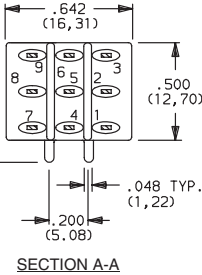
E301MD1AV2BE Vertical Actuation 3PDT
