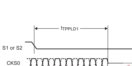
Figure 23. PLL Power-Down Time
