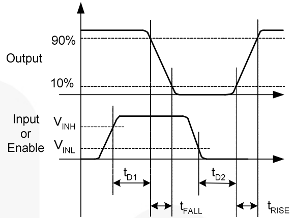
Figure 9. Inverting
