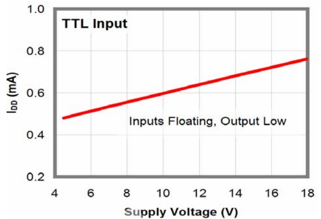
Figure 11. I_{DD} (Static) vs. Supply Voltage (12)
