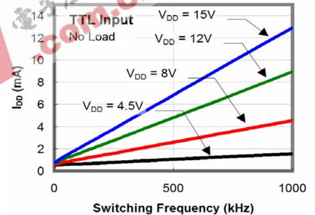
Figure 13. I_{DD} (No-Load) vs. Frequency
