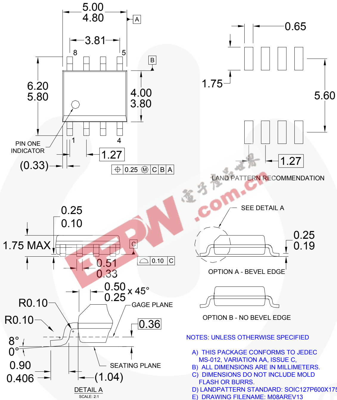
Figure 56. 8-Lead SOIC
