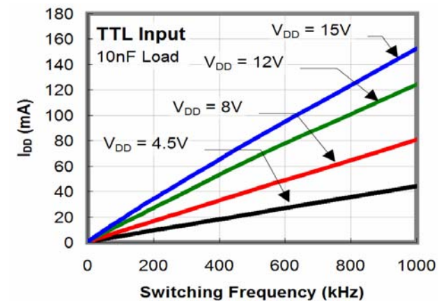
Figure 15. I_{DD} (10nF Load) vs. Frequency
