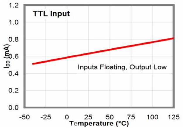
Figure 17. I_{DD} (Static) vs. Temperature (12)
