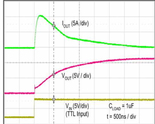
Figure 41. Quasi-Static Source Current with V_{DD}=12V (13)
