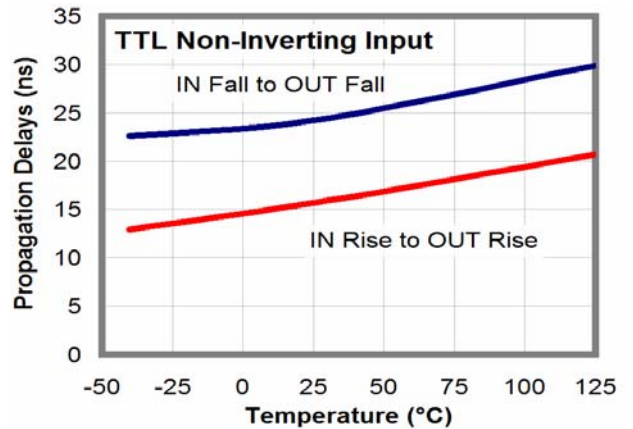
Figure 33. Propagation Delays vs. Temperature
