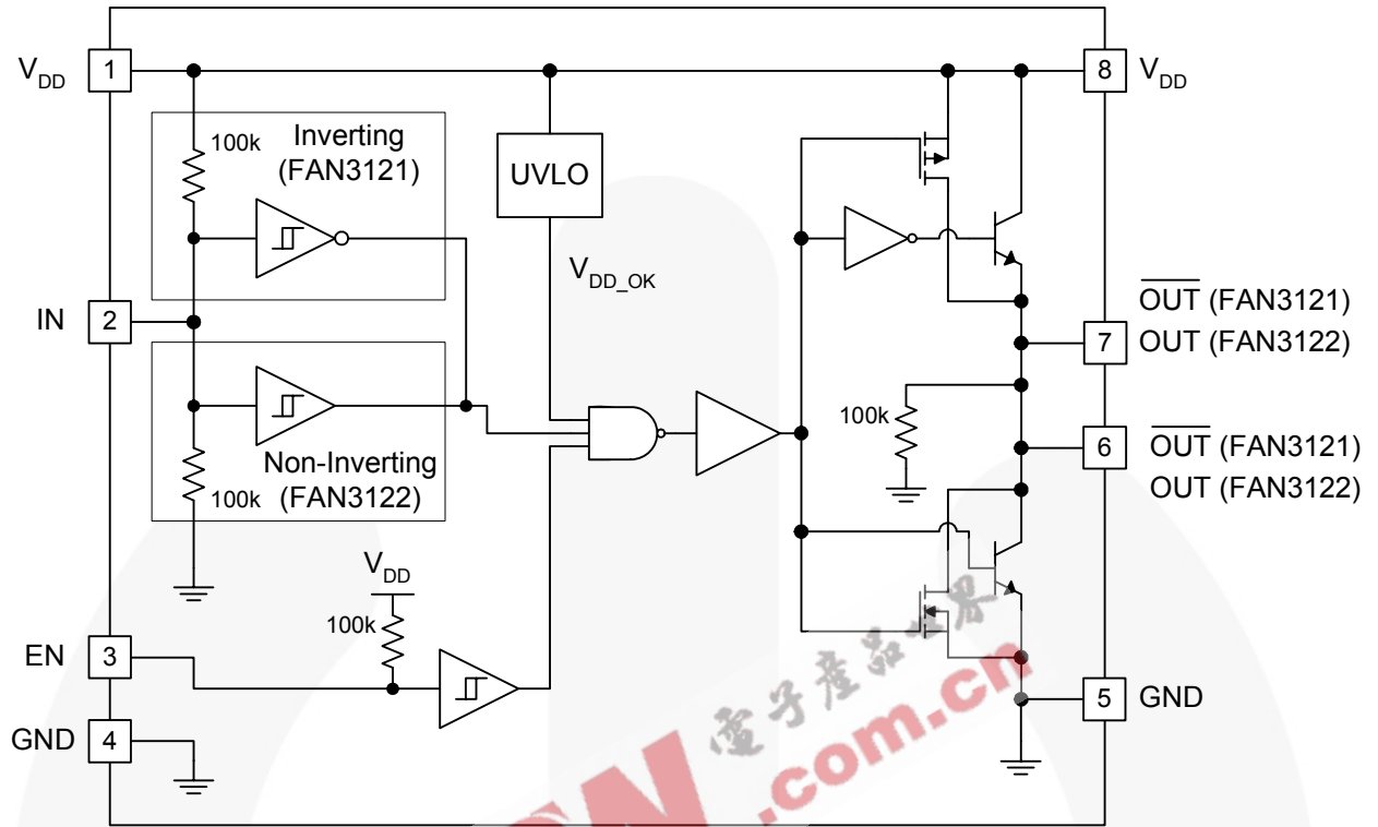
Figure 7. Block Diagram
