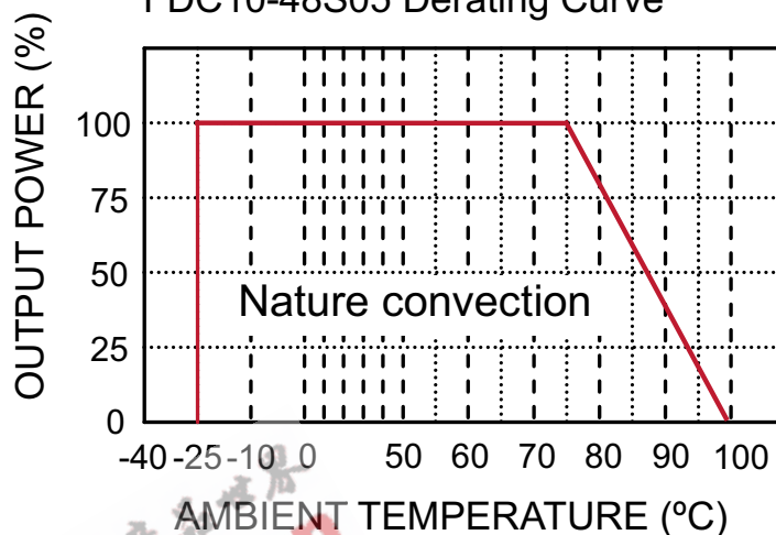
FDC10-48S05 Derating Curve
