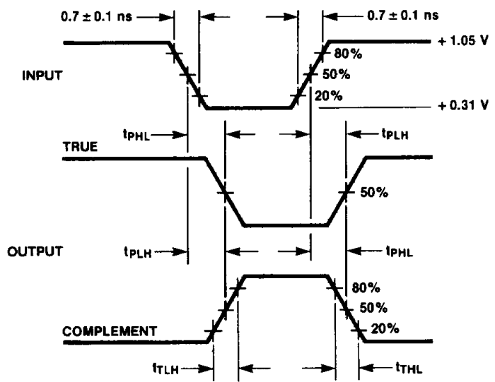
FIGURE 2. Propagation Delay and Transition Times
