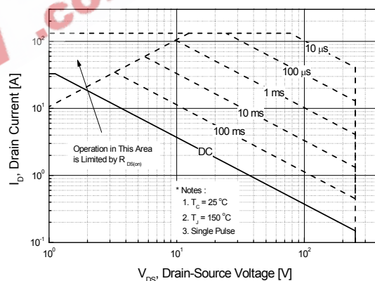
Figure 9-2. Maximum Safe Operating Area for FDPF33N25
