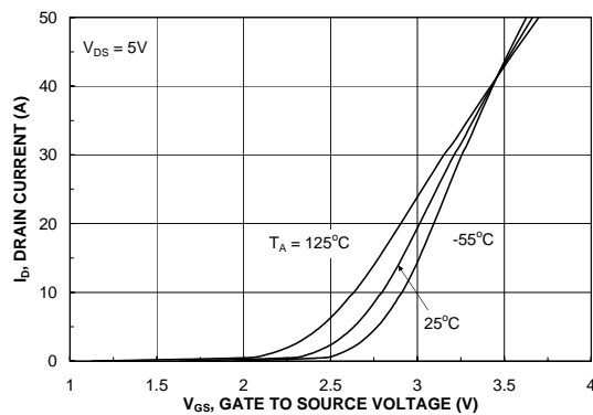
Figure 19. Transfer Characteristics.
