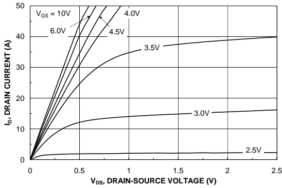
Figure 15. On-Region Characteristics.
