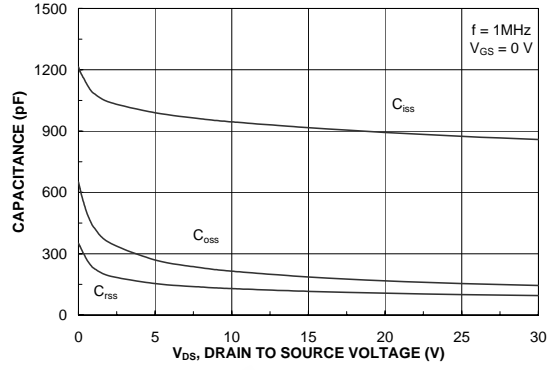
Figure 22. Capacitance Characteristics.
