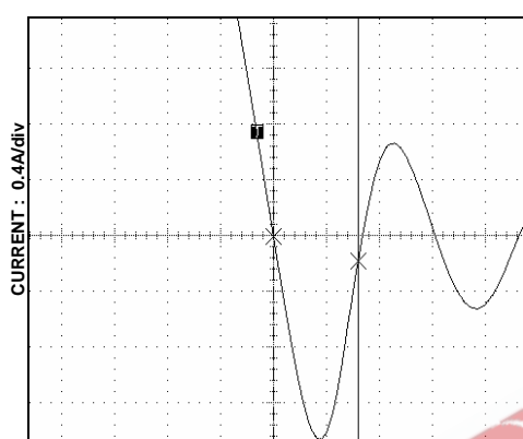
Figure 12. FDS6670AS SyncFET body diode reverse recovery characteristic.
