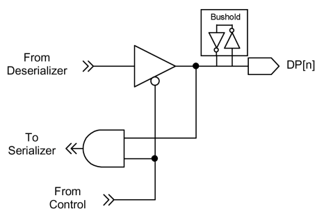
FIGURE 6. LVC MOS I/O
