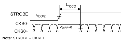
FIGURE 20. Serializer Clock Propagation Delay
