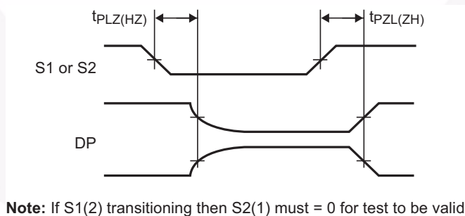
Figure 15. Deserializer Enable and Disable Times
