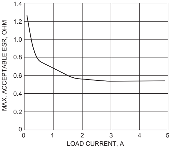
FAN1581 Stability
