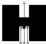
a) 42^\circ\text{C/W} when mounted on a 1\text{in}^2 pad of 2 oz copper
