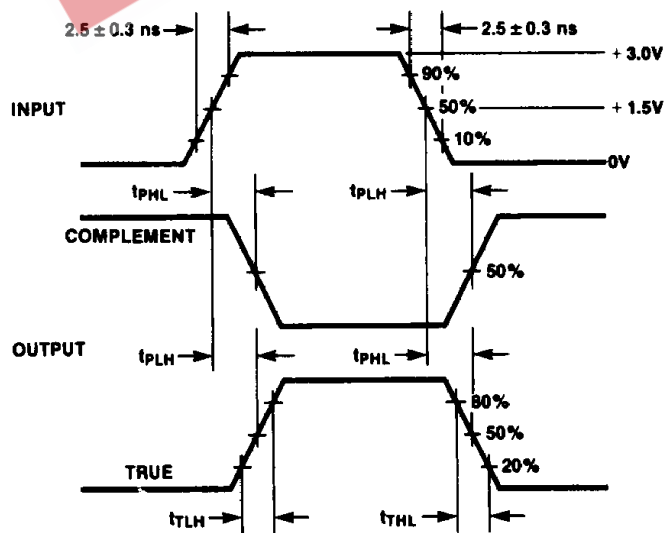
FIGURE 2. Propagation Delay and Transition Times
