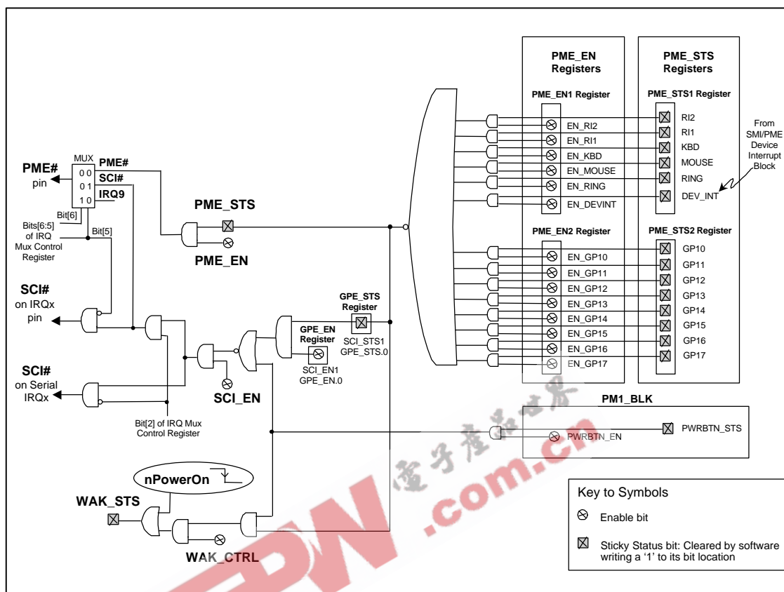
FIGURE 7 - PME/SCI LOGIC
