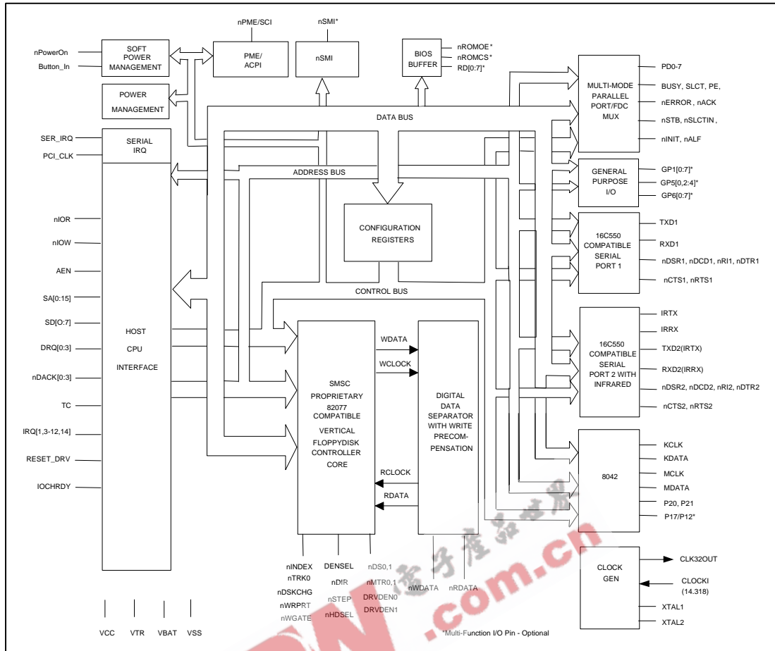
FIGURE 2 - FDC37B72x BLOCK DIAGRAM
