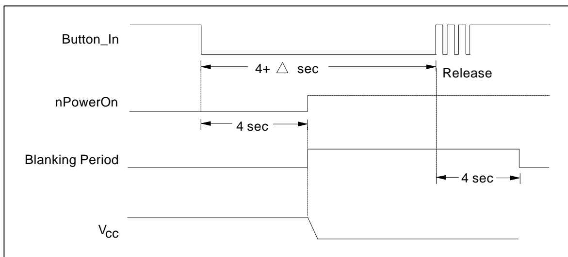
FIGURE 6 - BLANKING PERIOD
