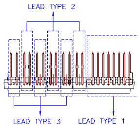
DETAIL LEAD
