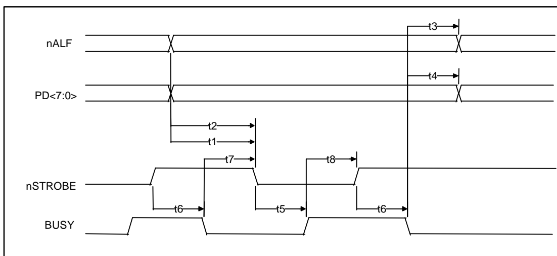
FIGURE 19 - ECP PARALLEL PORT FORWARD TIMING
