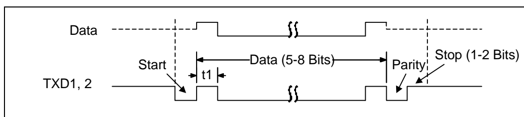
FIGURE 12A - SERIAL PORT DATA
