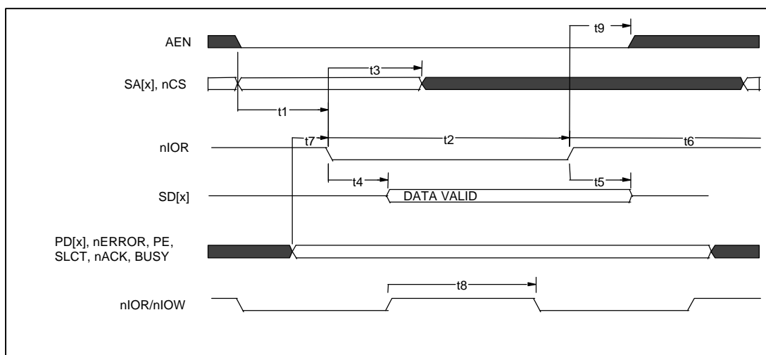
FIGURE 7 - ISA READ
