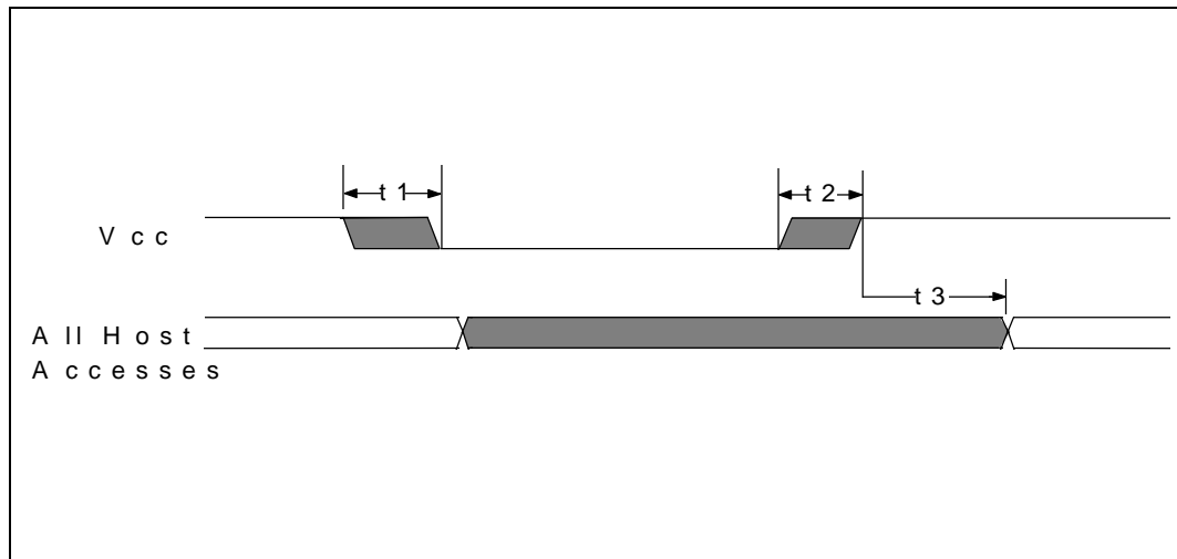
FIGURE 5 - POWER-UP TIMING
