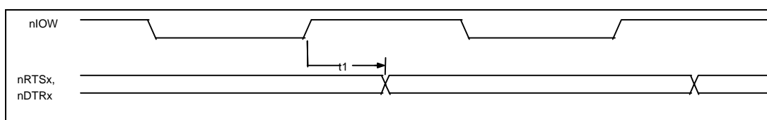
FIGURE 12 - SERIAL PORT TIMING
