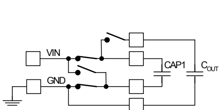
Figure 10. 2:1 Charge Pump Configuration V_{OUT} = 2 \times V_{IN}
