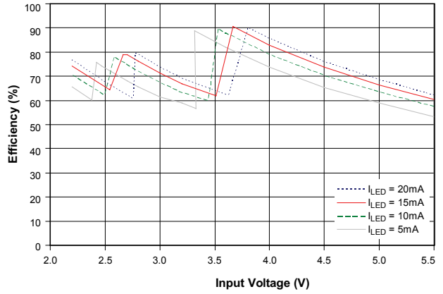
Figure 4. Efficiency vs. Input Voltage
