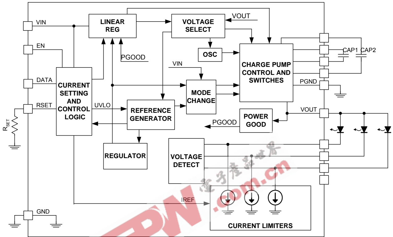
Figure 9. IC Block Diagram
