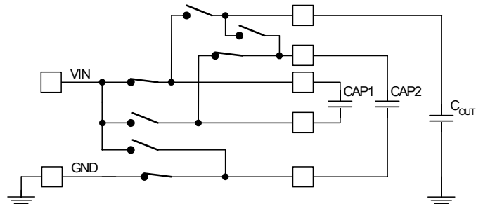
Figure 11. 3:2 Charge Pump Configuration V_{OUT} = 1.5 \times V_{IN}
