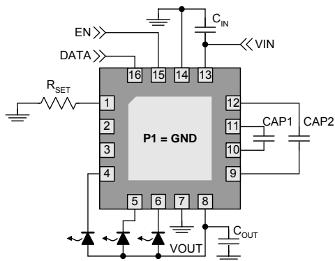
Figure 1. Typical Application
