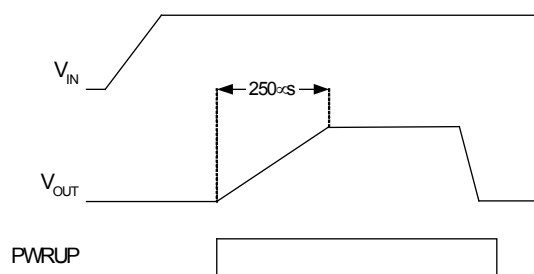
Figure 12. Soft-Start
