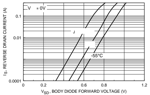
Figure 6. Voltage Variation with Source Current and Temperature.
