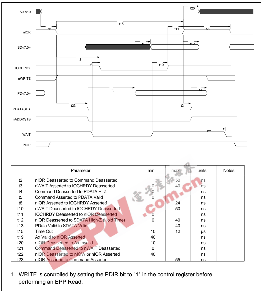
FIGURE 16 - EPP 1.7 DATA OR ADDRESS READ CYCLE
