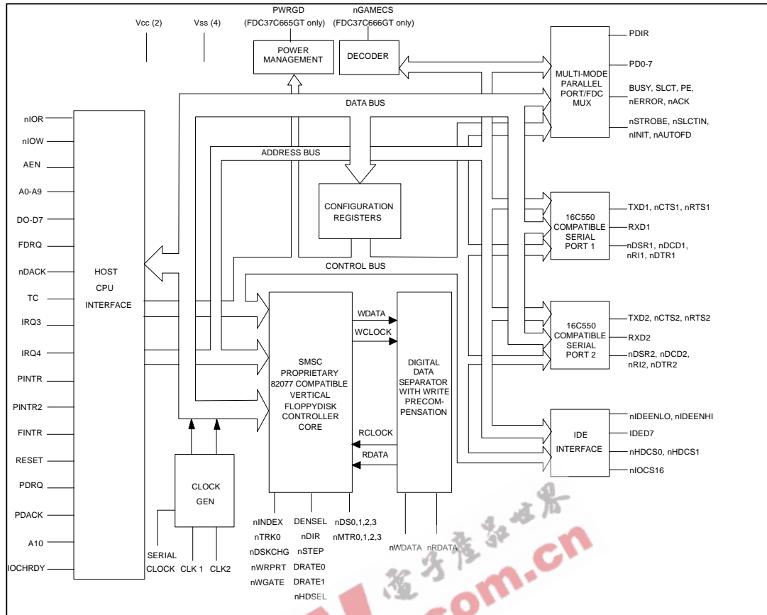
FIGURE 1 - FDC37C665GT/FDC37C666GT BLOCK DIAGRAM
