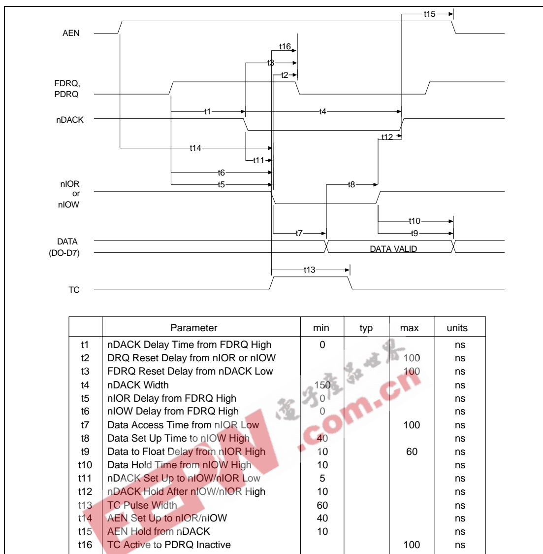
FIGURE 6 - DMA TIMING
