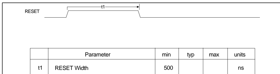
FIGURE 7 - RESET TIMING
