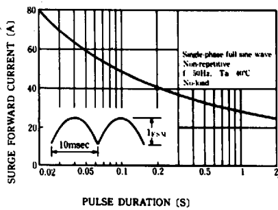
FIG.4-SURGE CURRENT RATINGS
