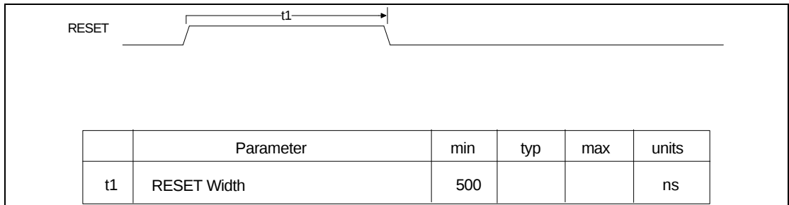
FIGURE 7 - RESET TIMING
