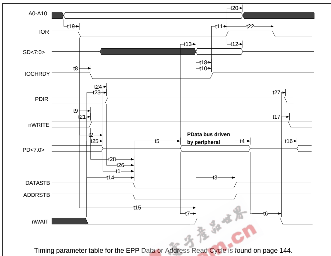
FIGURE 14A - EPP 1.9 DATA OR ADDRESS READ CYCLE
