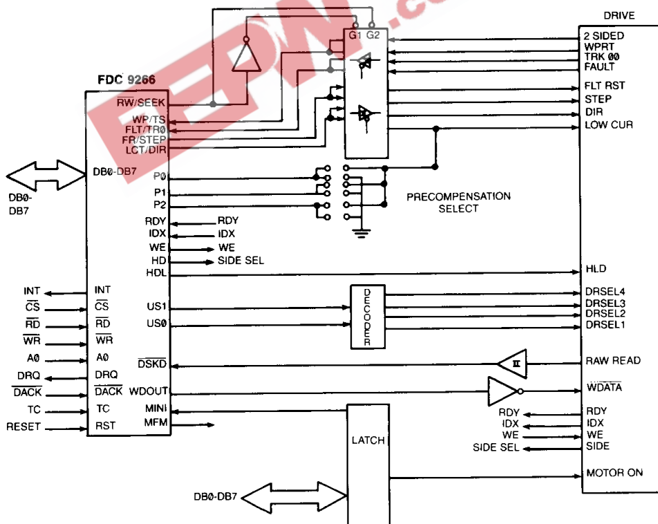
TYPICAL APPLICATION
