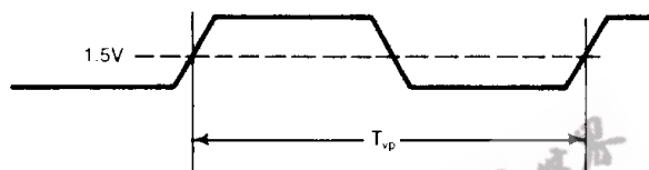
FIGURE 1: VCOCLK TIMING
