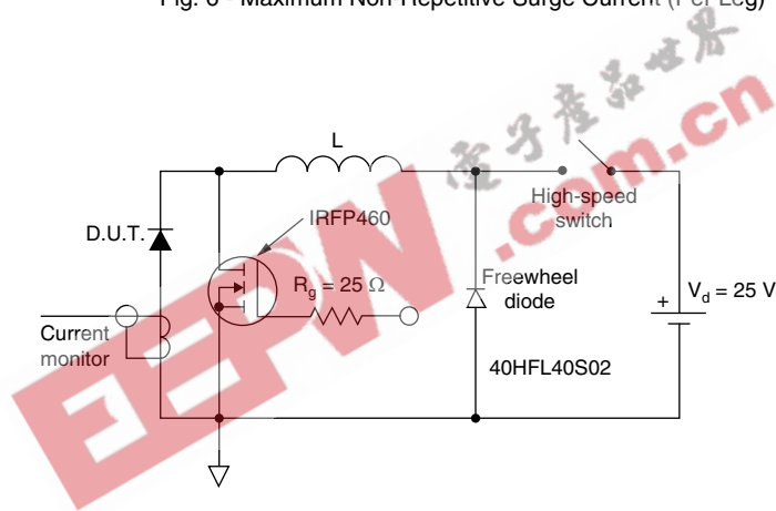
Fig. 7 - Unclamped Inductive Test Circuit
