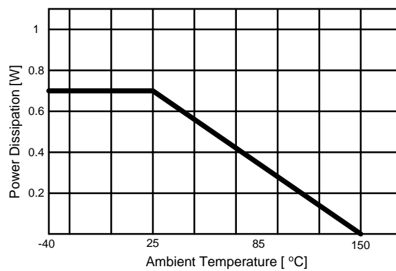
Figure 14. Power derating curve
