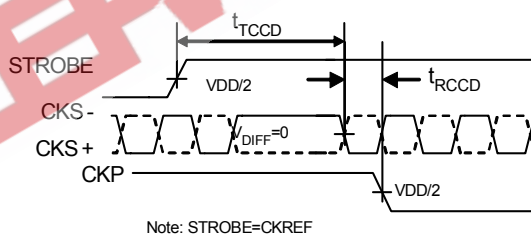
Figure 9. Clock Propagation Delay
