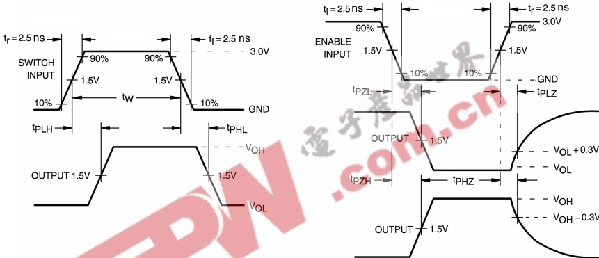
FIGURE 3. AC Waveforms
