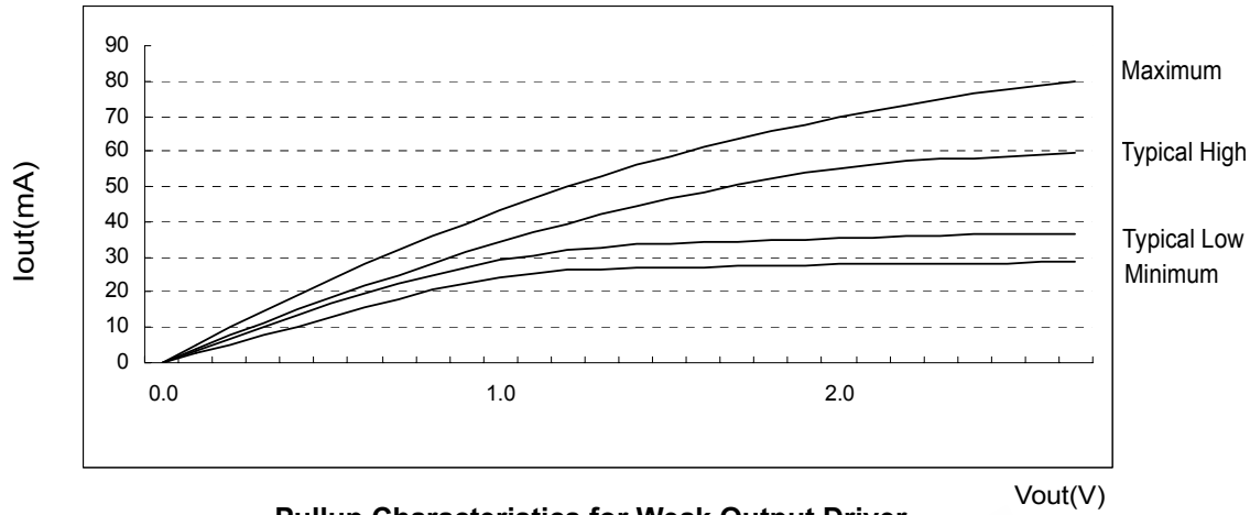
Pullup Characteristics for Weak Output Driver
