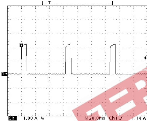
Short Circuit-Current
