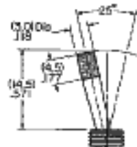
C .571" Color Tipped Cone (available on 1 & 2-pole only)
