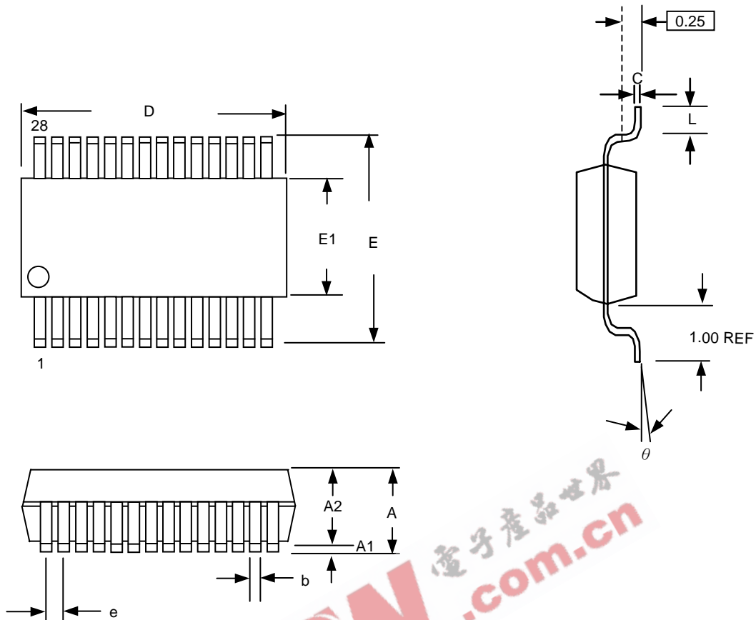
SSOP-28 Package
