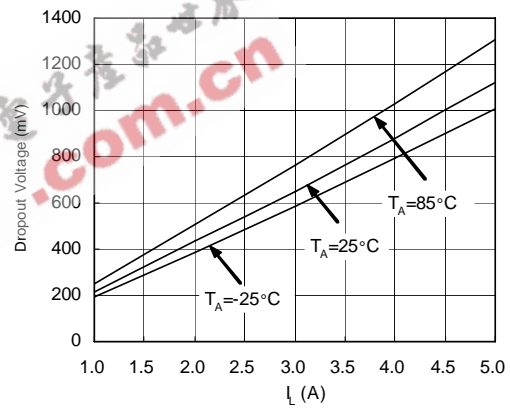
G1084-33 Dropout Voltage vs. I_L
