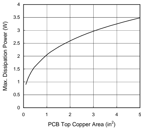
G1084T43(TO-252) Max. Power Dissipation vs. PCB Top Copper Area T_{\text{AMB}} = 25^{\circ}\text{C} ; Still Air
