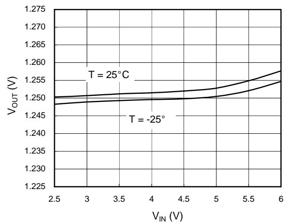
Line Regulation
