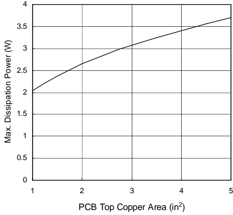
G1084T53(TO-263) Max. Power Dissipation vs. PCB Top Copper Area Area T_{AMB} = 25^{\circ}C ; Still Air
