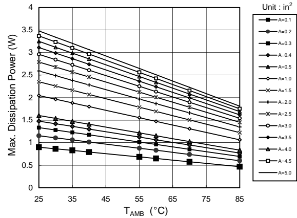
G1084T43(TO-252) Max. Power Dissipation vs. T_{\text{AMB}} (still air) (Different PCB Top Copper Area)
