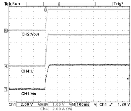
G1085-18-Start-up
