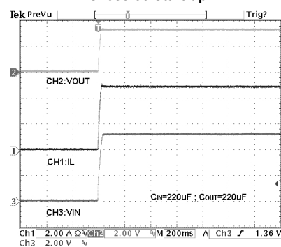
G1085-33 Start-up
