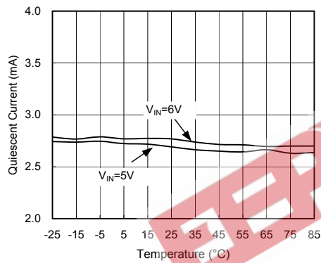
G1085-33 Quiescent Current vs. Temperature
